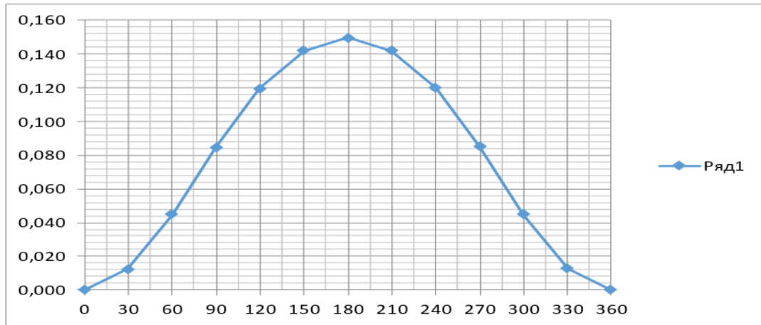
3-rasm. Ichki yonuv dvigatelining chiqish zvenosining siljish diagrammasi
