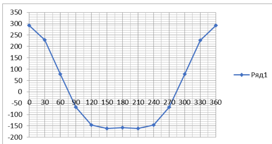
5-rasm. Ichki yonuv dvigatelining chiqish zvenosining tezlanish diagrammasi
