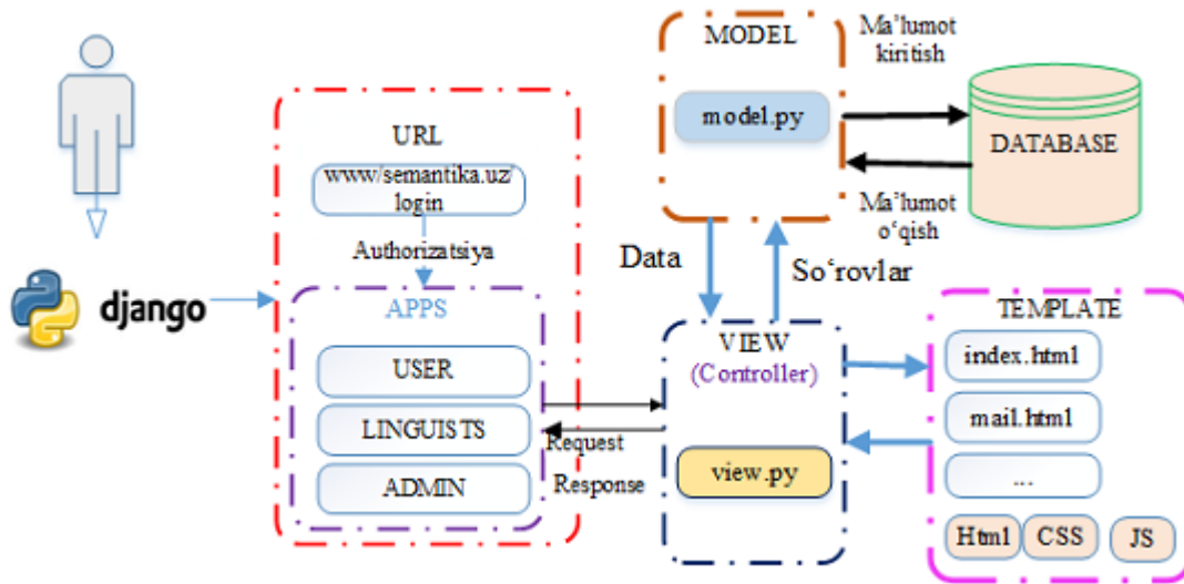
Fig. 4. Information system architecture
