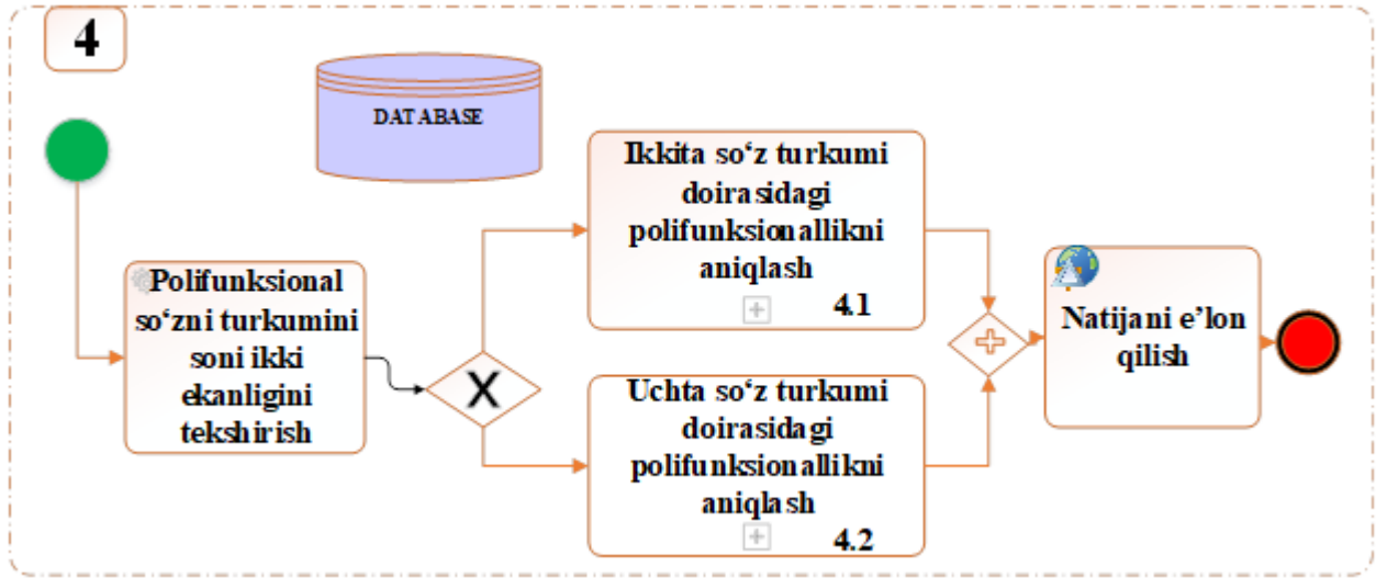
Fig. 3. The process of determining in which part of speech a polyfunctional word can be found
