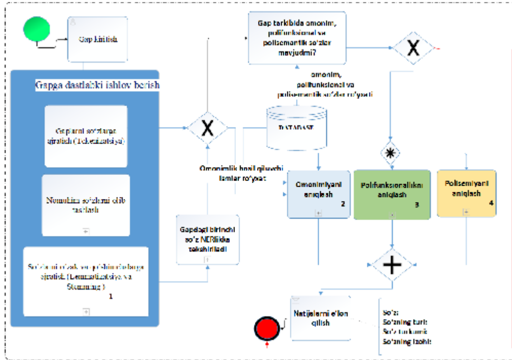
Fig. 2. BPM model of general information system processes.
